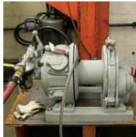
Air Winch on Line Pull Test
