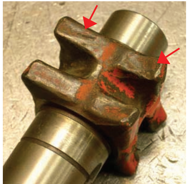
High wear on a hoist's chain guide can cause the chain to slip or the hoist to lock up under load. This can also indicate significant side loading.
